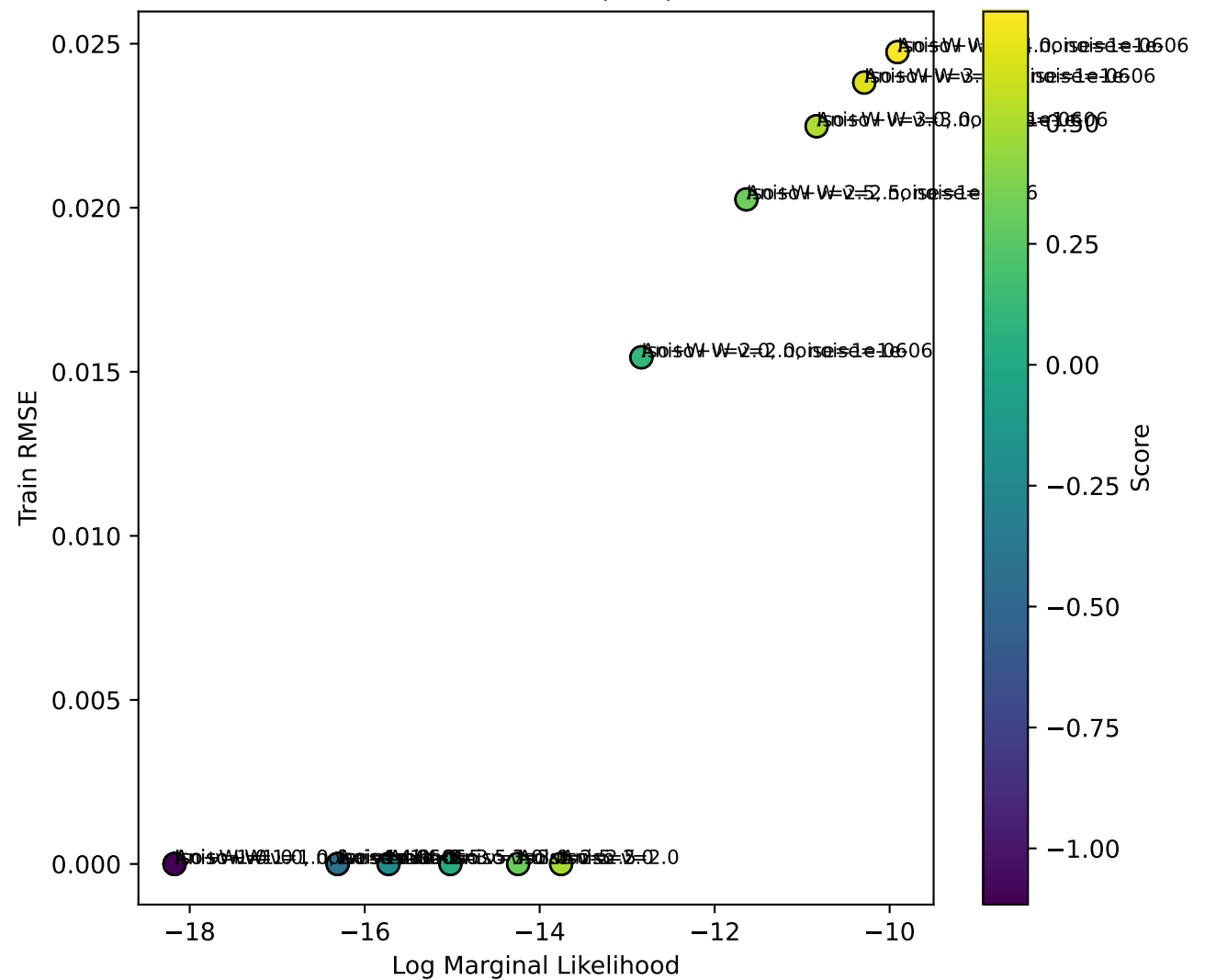
LML vs RMSE (T13)
