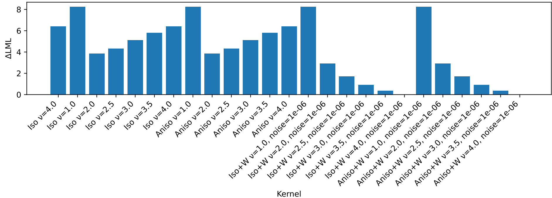
Difference from best LML (T13)
